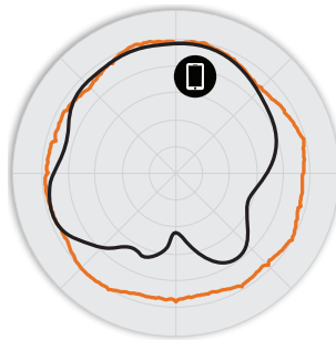
Figure 3. R310 5GHz Azimuth Antenna Patterns
